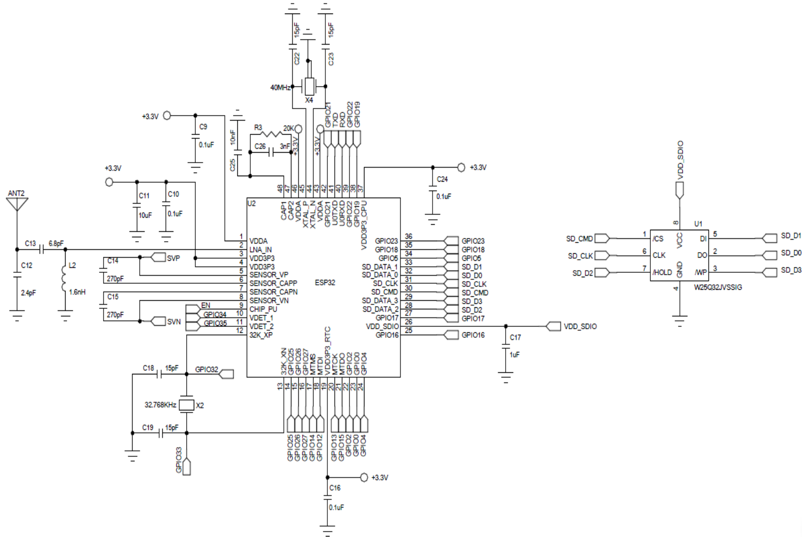
Chart 22: Hardware Schematics
