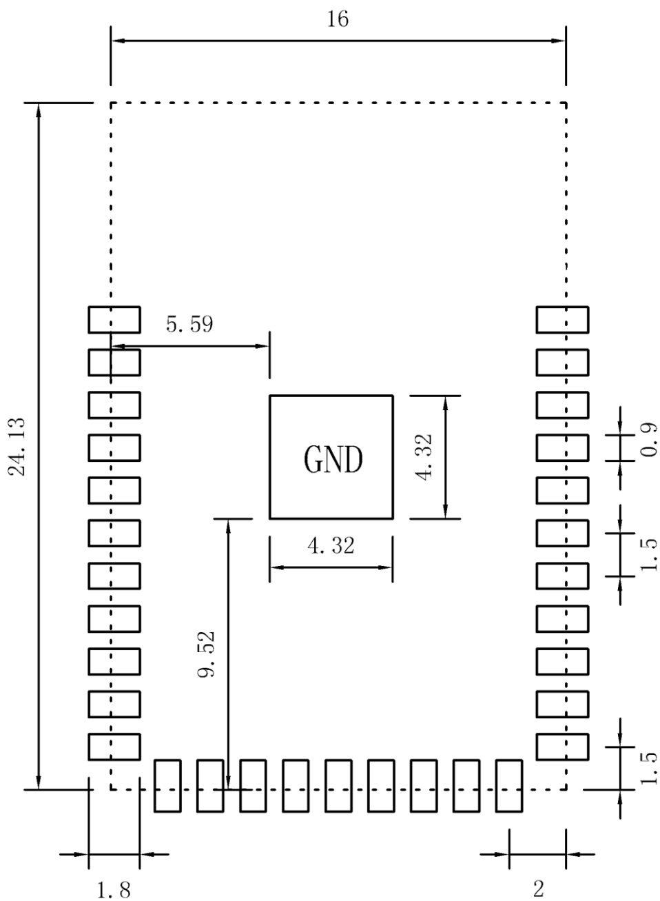
Chart 18: Fig.3-Recommended PCB Layout (Top View, Unit: mm)
