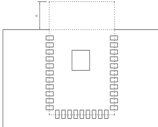
Chart 19: Fig.4-Module Layout Scheme 1(antenna is out of the frame, Unit: mm)
